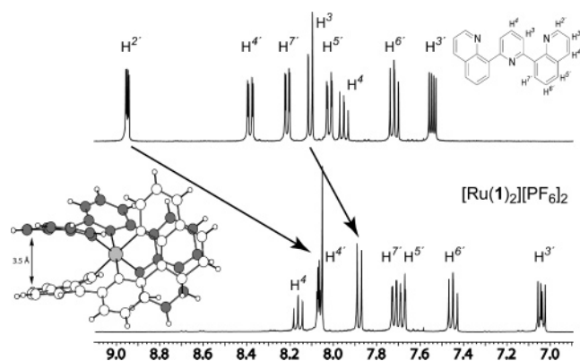
FIGURE 2. Ball and stick representation of [\text{Ru}(\mathbf{1})_2][\text{PF}_6]_2 and ^1\text{H} NMR spectra of 1 (top) and [\text{Ru}(\mathbf{1})_2][\text{PF}_6]_2 (bottom) in \text{CD}_3\text{CN} .
