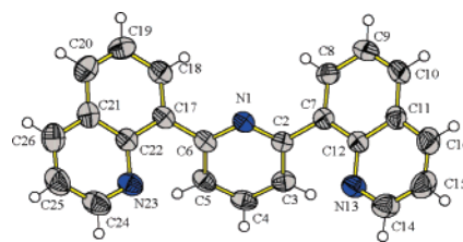
FIGURE 1. ORTEP view of 1 at 50% probability level.
